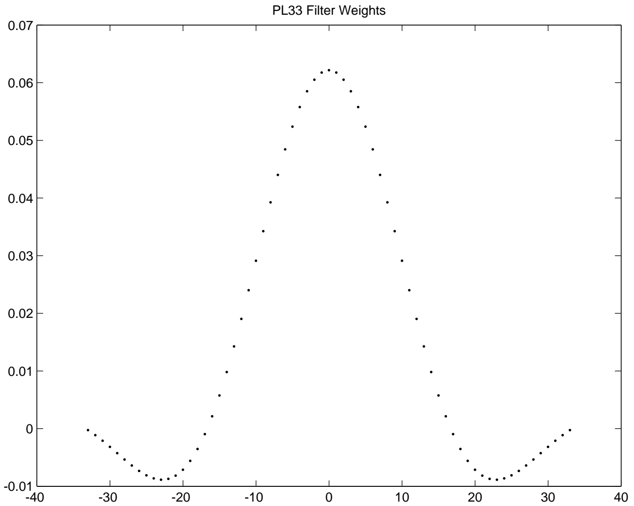
Figure 47: Filter weights applied to the time-series data in the low-pass filter PL33. The filter truncates 33 points from the beginning and end of each time series.
