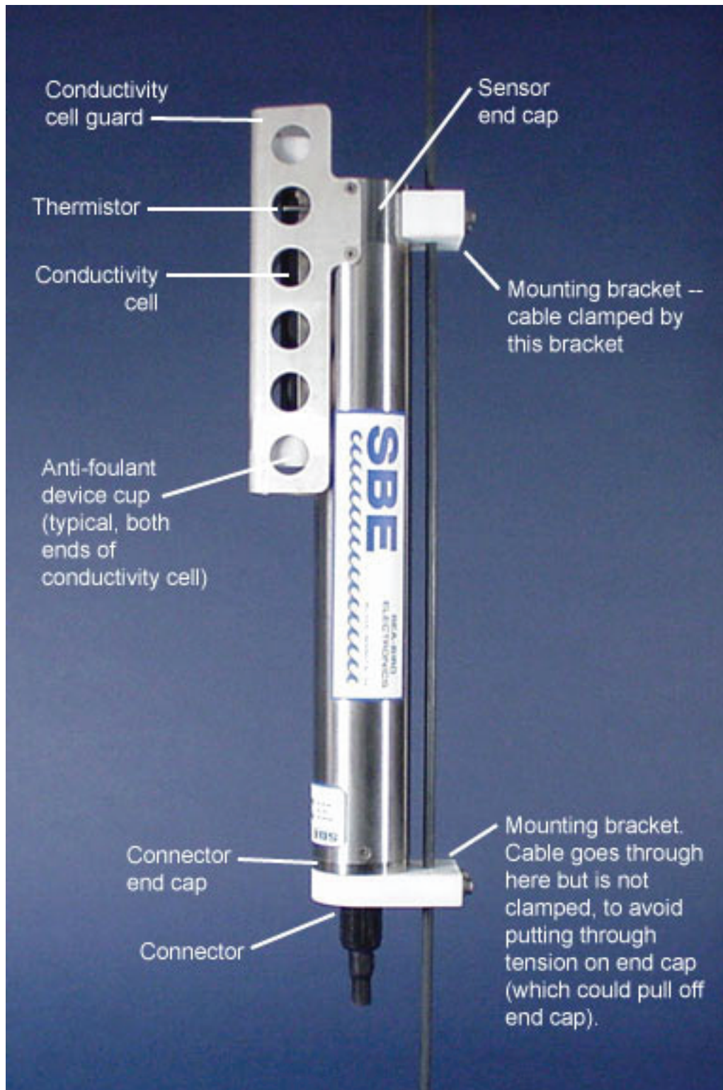
Figure 25. A photograph of a MicroCAT conductivity and temperature sensor manufactured by Sea-Bird Electronics. The conductivity and temperature sensors are located under the conductivity cell guard as seen in the photo. This photo is courtesy of Sea-Bird Electronics.
