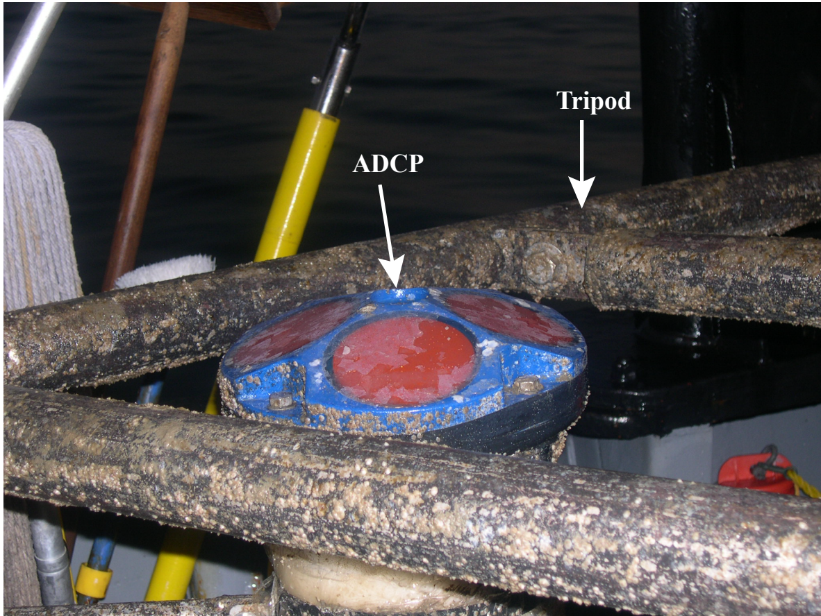
Figure 33. A photograph of the tripod recovered from Site 2 at the end of the second deployment. Biofouling was significantly less during the second deployment, as seen in this photograph where the surfaces of the tripod and the ADCP have minimal fouling.
