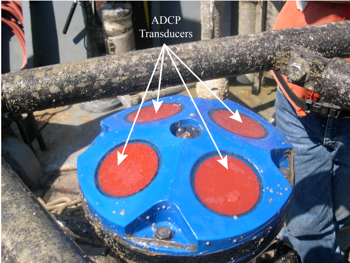
Figure 35. A photograph of the ADCP on the tripod recovered from Site 3 at the end of the second deployment. Biofouling was much less significant during this deployment. The ADCP transducers are free from any biofouling.
