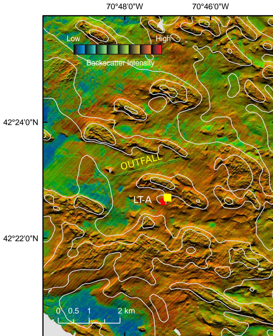
Figure 7. Map showing location of tripod moorings (over-lapping red triangles) at LT-A in western Massachusetts Bay. The yellow square is the location of the U.S. Coast Guard B buoy. The locations are plotted on a map of shaded-relief bathymetry colored by backscatter intensity (Butman and others, 2003; Butman and others, 2007b). Backscatter intensity is a measure of surface sediment texture and bottom roughness. Generally, high backscatter intensity (shown as red and yellow) is associated with rock outcrops, gravel, and coarse-grained sediment, medium backscatter intensity (green) is associated with sandy sediments, and low backscatter intensity (shown as blue) indicates finer grained sediments. The tripods are located in an area of moderate to high backscatter intensity in about 30 m water depth on the southern flank of a ridge that runs approximately northwest-southeast. The Massachusetts Water Resources Authority (MWRA) ocean outfall appears as two parallel rows (about 2 km long) of individual mounds of material; the mounds are rock materials discarded on the sea floor from the holes drilled for the risers that extend to the outfall tunnel below. The diffuser heads, about 3 m high and 4 m in diameter and located between the rows, are not resolved in this image. For a map of a larger area around the mooring site, see Butman and others (2003).
